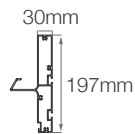
⑧ Motorbox Support Bar
