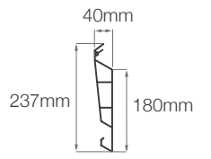
⑤ Louvre
